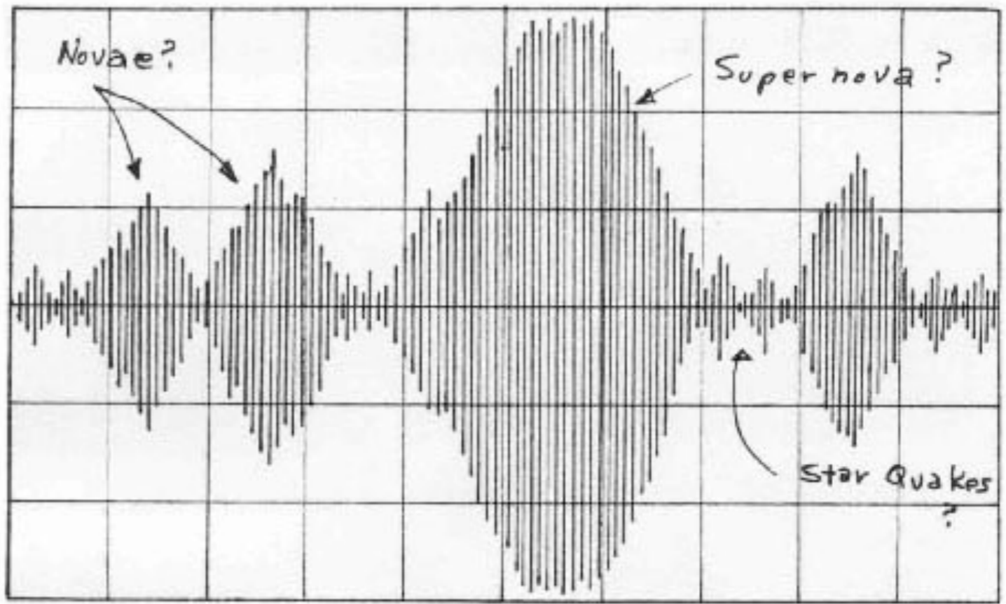
(a) Typical Nova Response
