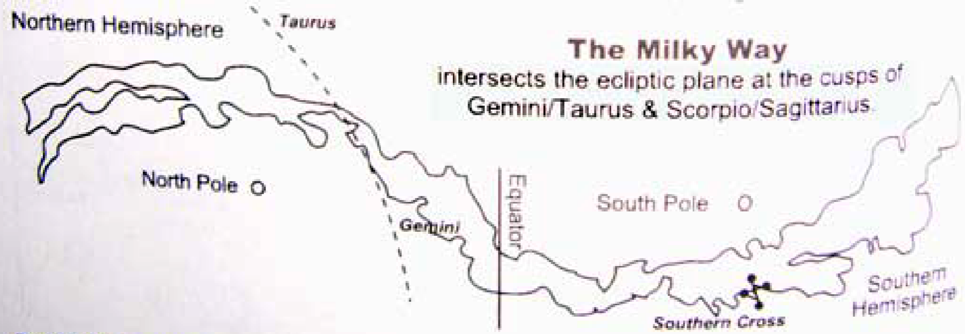
Figure 12.2. The alignment of the ecliptic, the solar cube of space and the galactic meridian. Note that the ecliptic crosses the galactic plane at the cusps of Gemini/Taurus and at the cusp of Scorpio/Sagittarius, as shown.
