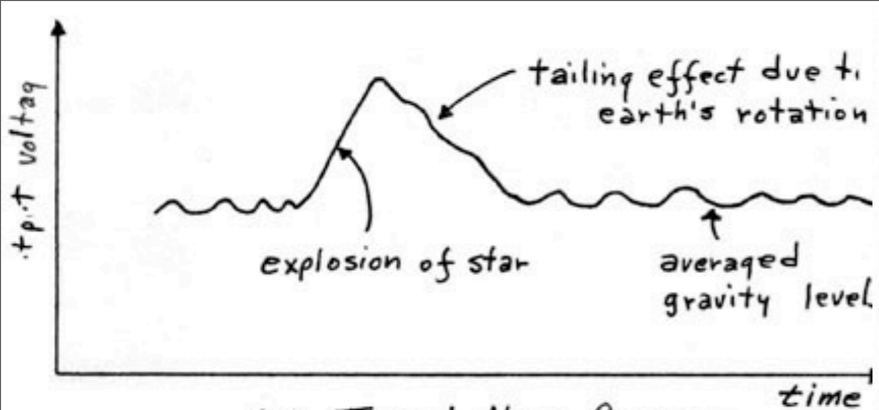
(a) Typical Nova Response
